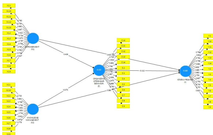
Gambar 2 Loading Factor
