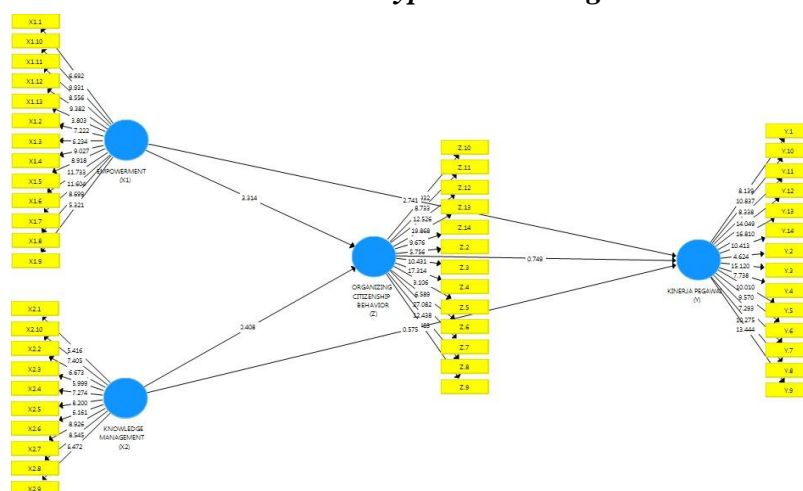
Gambar 5 Hypotesis Testing
